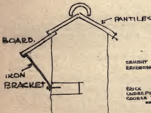
WALL COPINGS.
